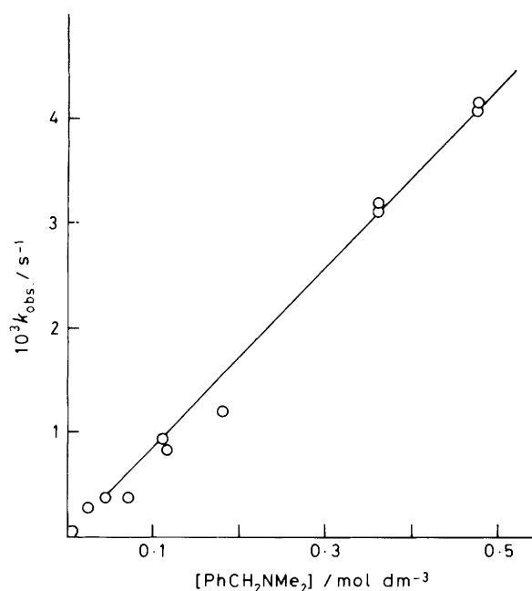
Figure 1. The dependence of k_{\text{obs}} on the concentration of NN -dimethylbenzylamine for palladation of the amine by [\text{Pd}_3(\text{O}_2\text{CMe})_6] in acetic acid at 50 °C
