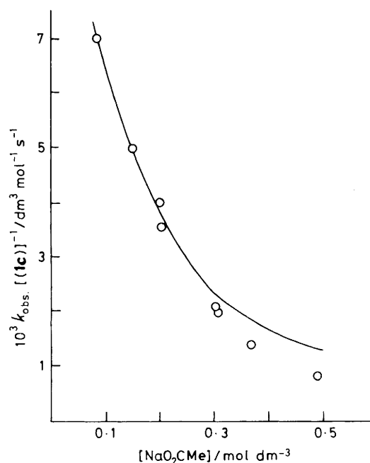
Figure 2. Plot of the second-order rate constant k_{\text{obs.}}/[(1c)] versus [\text{NaO}_2\text{CMe}] for palladation of NN -dimethylbenzylamine by \text{Na}_2\text{[Pd}_2(\text{O}_2\text{CMe})_6] in acetic acid at 50 °C
