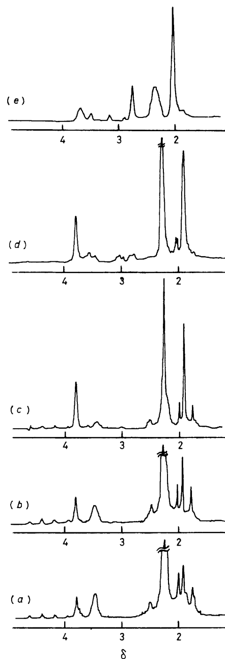
Figure 4. Interaction of 1 molar equivalent palladium(II) acetate with 2 molar equivalents of NN -dimethylbenzylamine in \text{CDCl}_3 as studied by ^1\text{H} n.m.r. spectroscopy. Spectra: (a) immediately after warming the frozen solution to -40^\circ\text{C} ; (b) after 35 min at -40^\circ\text{C} ; (c) after increasing the temperature to 0^\circ\text{C} ; (d) after 30 min at 0^\circ\text{C} ; (e) at 30^\circ\text{C} . For details see text
