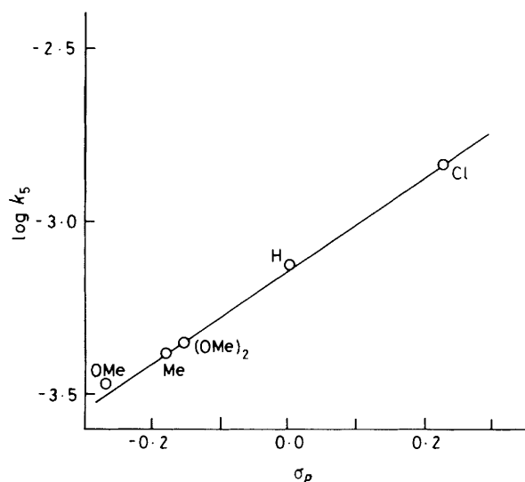
Figure 3. Hammett plot of \log k_5 versus \sigma_p
