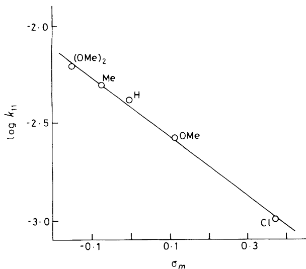
Figure 6. Hammett plot of \log k_{11} against \sigma_m
